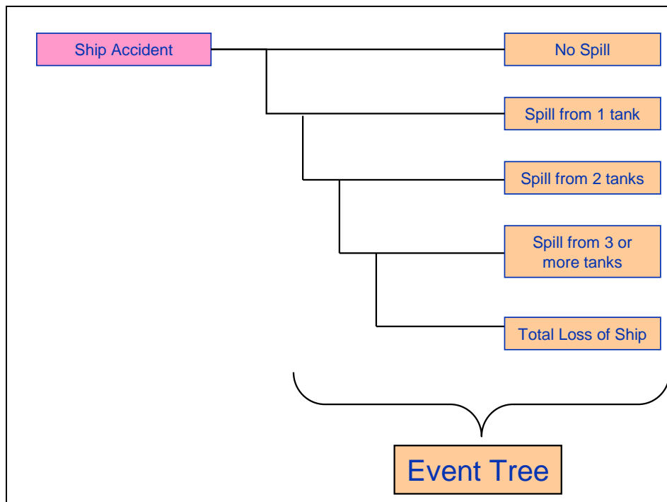
Figure 4-1 Generic Oil Outflow Event Tree
