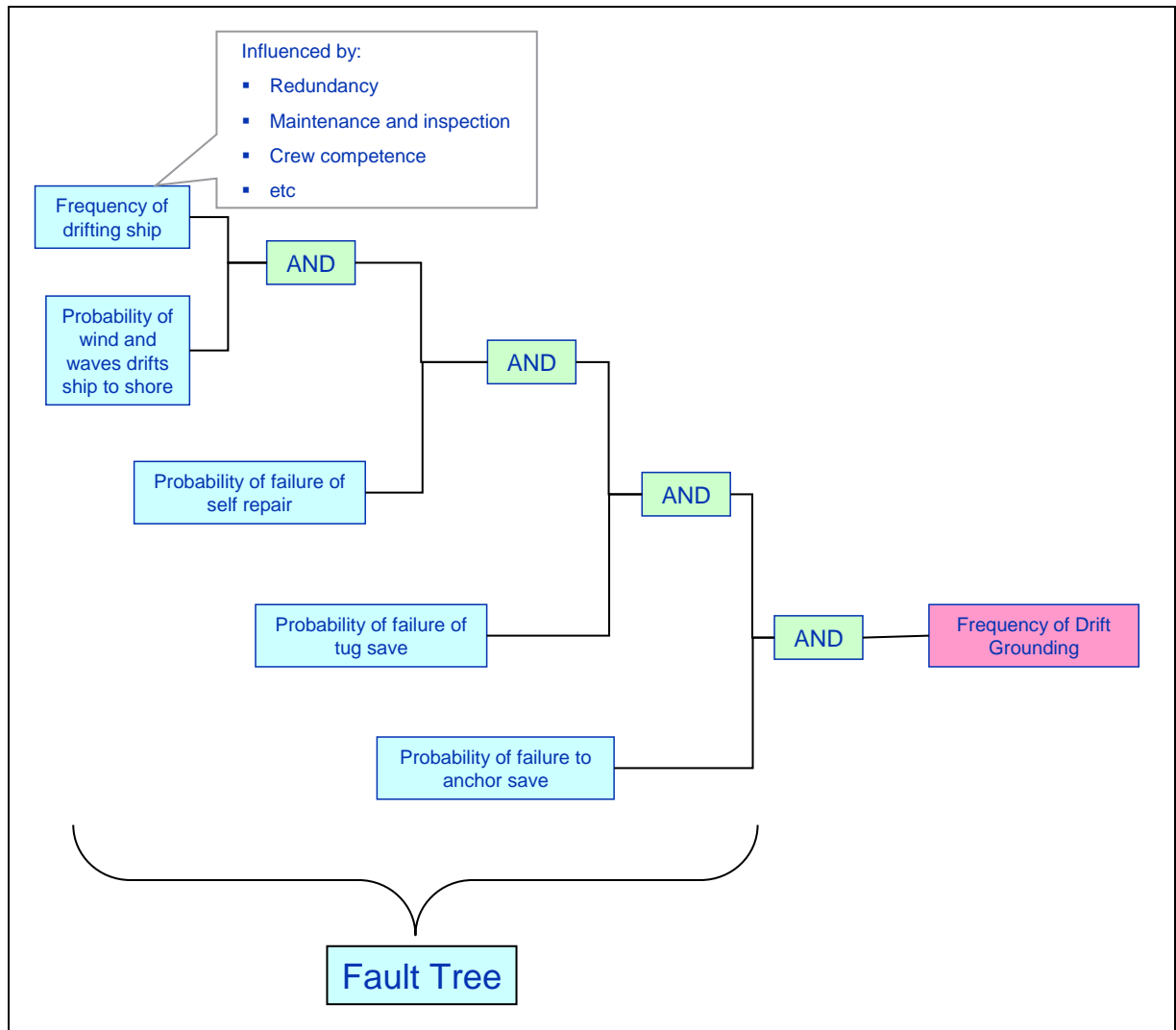
Figure 5-2 Drift Grounding Fault Tree
