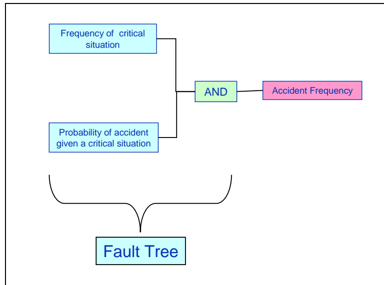
Figure 5-1 Generic Accident Frequency Fault Tree Used by MARCS
